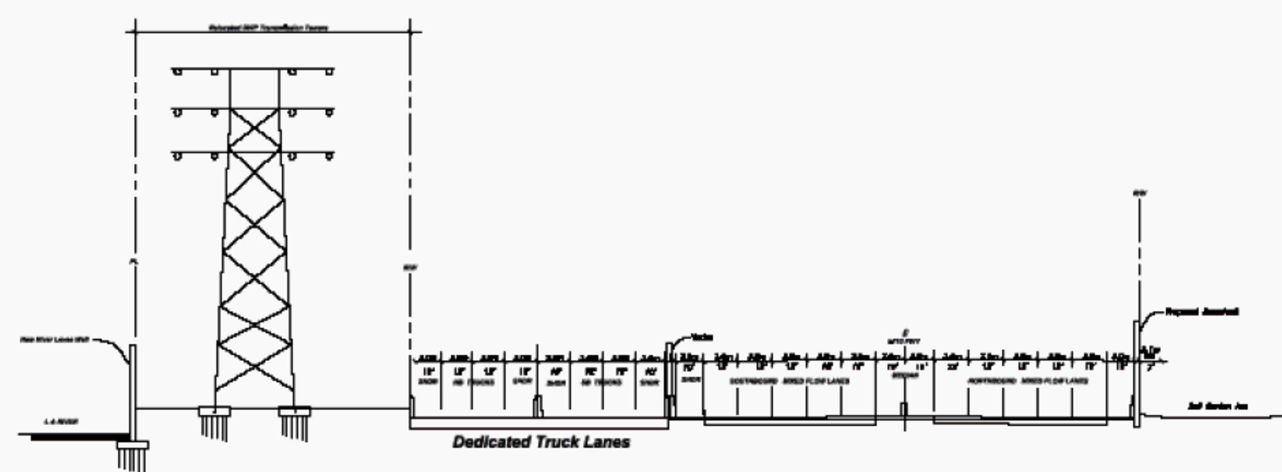
TYPICAL SECTION (Firestone Blvd to Florence Ave)
